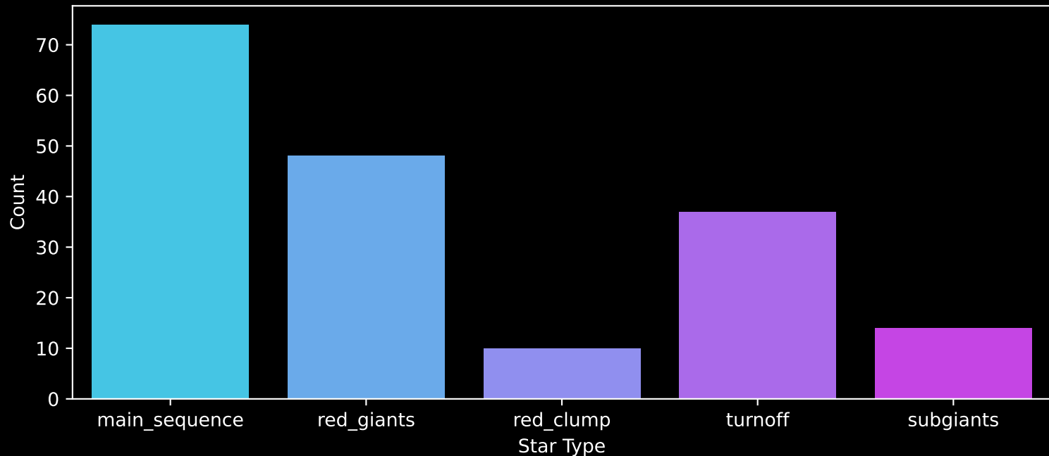
APOGEE DR17 Field: [269-30-O_TESS] Count plot of Star Type
