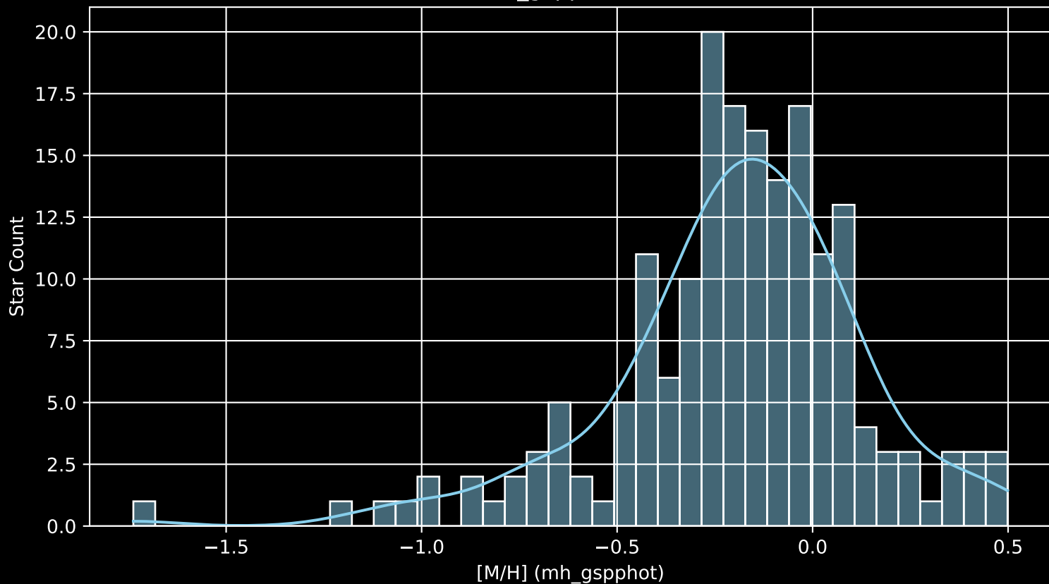
APOGEE DR17 Field: [269-30-O_TESS [M/H] (mh_gspphot) (n= 182)
