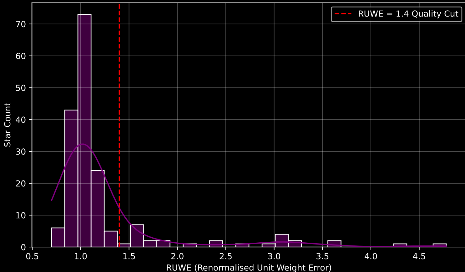
GAPOGEE DR17 Field [269-30-O_TESS] RUWE Distribution (n= 178)
