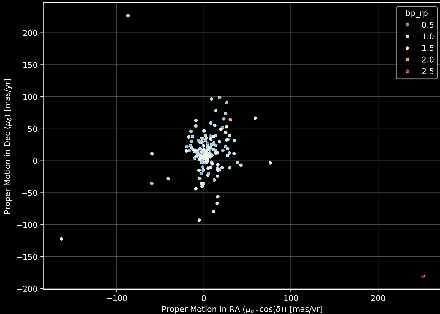
APOGEE DR17 Field: [269-30-O_TESS] Proper Motion Diagram (n= 183)
