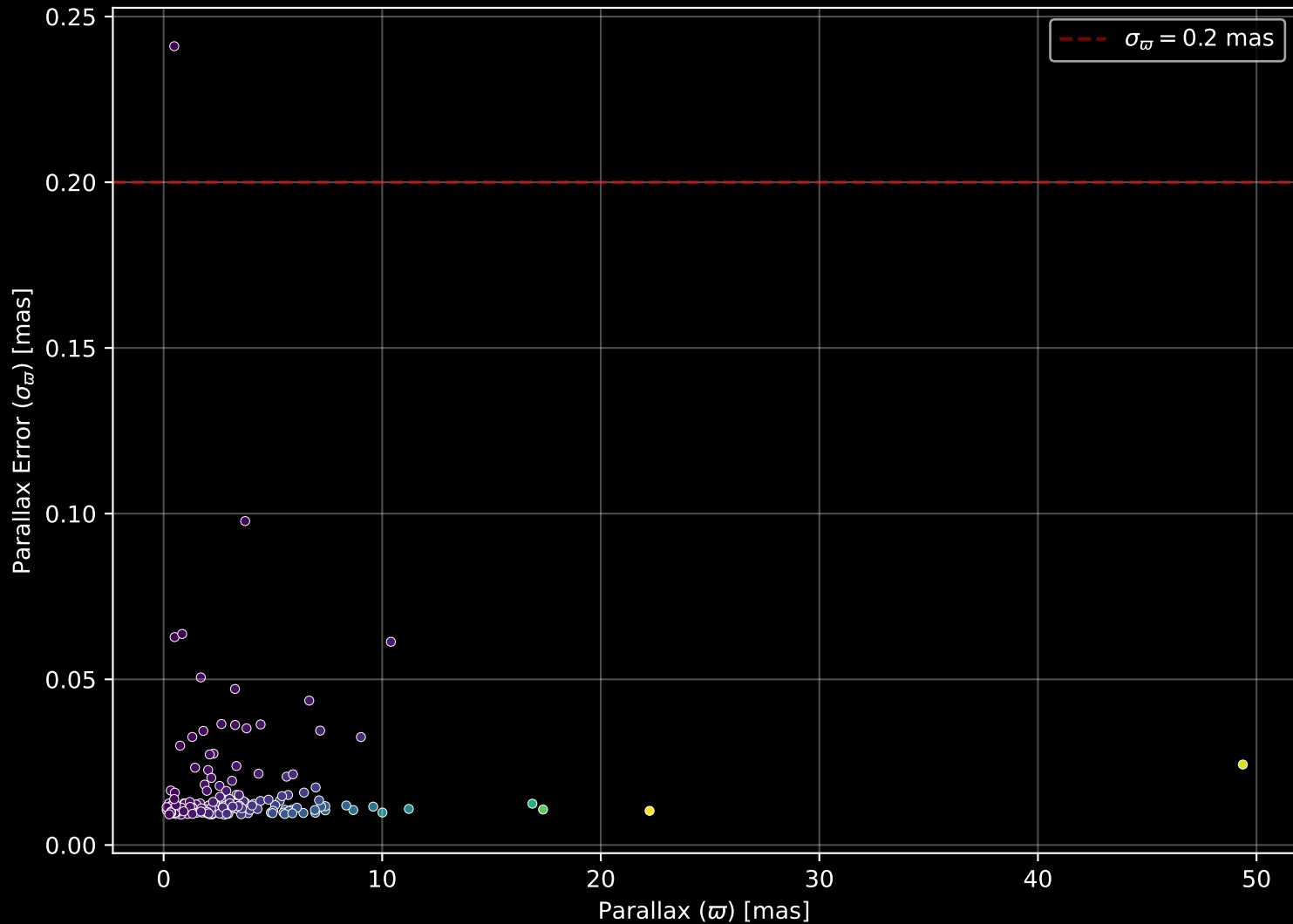
APOGEE DR17 Field: [269-30-O_TESS] Parallax Quality (n= 183)
